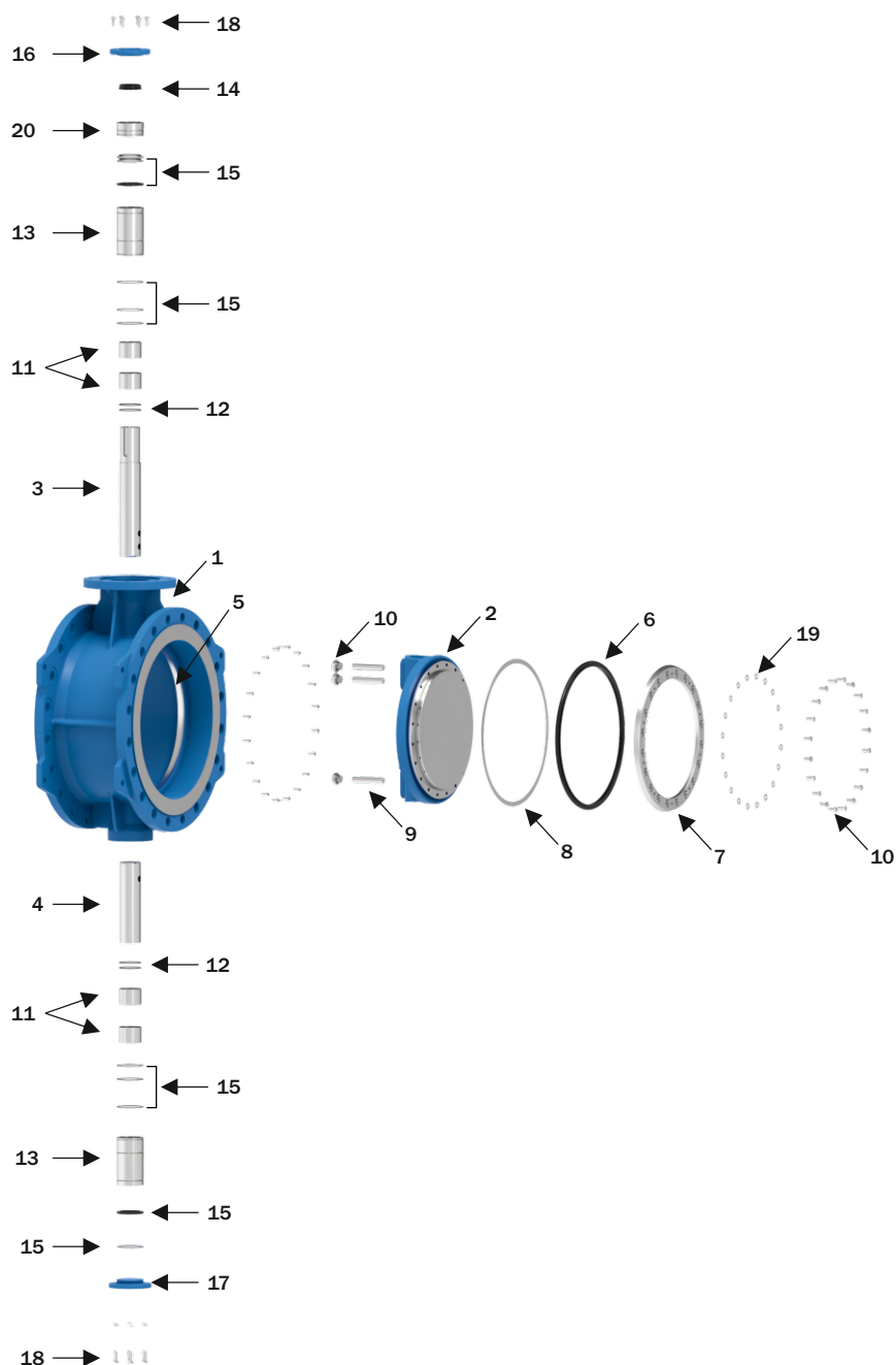
Component List - Dry Shaft
